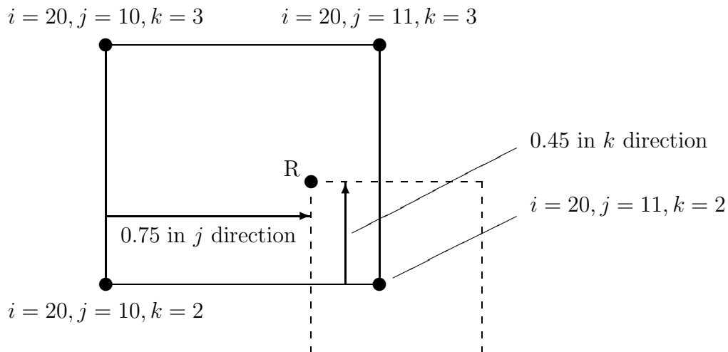
Figure 6: Example Interface for Generalized Connectivity, Structured Grids
