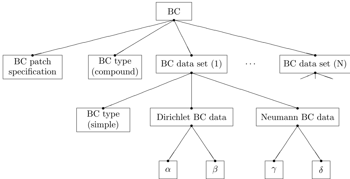
Figure 9: Hierarchy for Boundary Condition Structures
