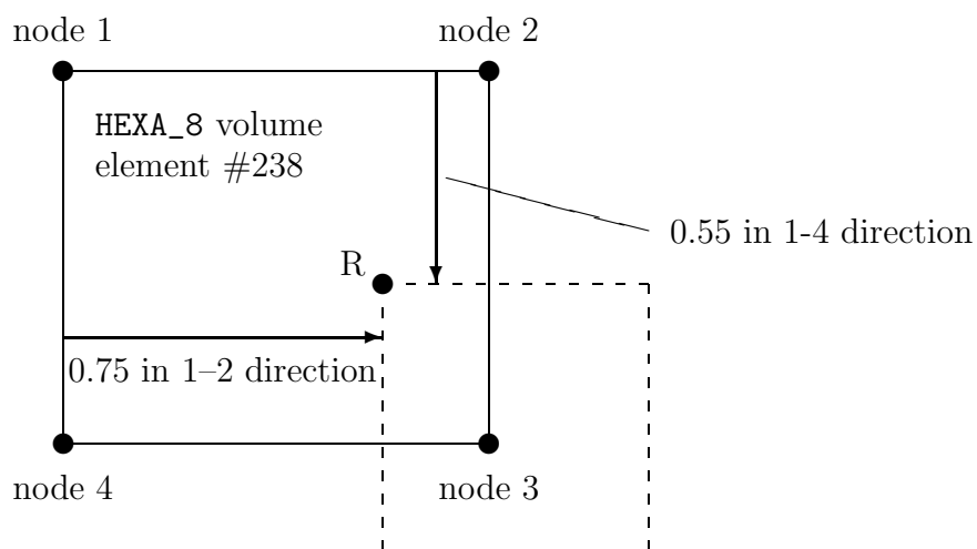
Figure 7: Example Interface for Generalized Connectivity, Unstructured Grids with HEXA_8 Donor Cell
