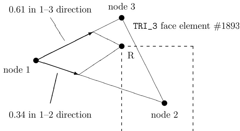
Figure 8: Example Interface for Generalized Connectivity, Unstructured Grids with TRI_3 Donor Cell
