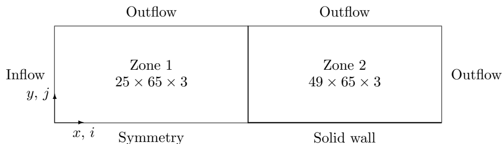
Figure B.1: Two-Zone Flat Plate Test Case
