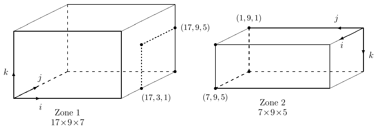
Figure 5: Example Interface for 1-to-1 Connectivity
