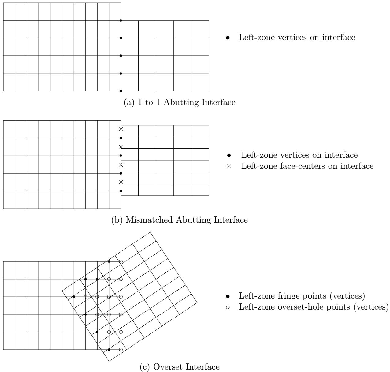
Figure 3: Structured-Grid Multizone Interface Types
