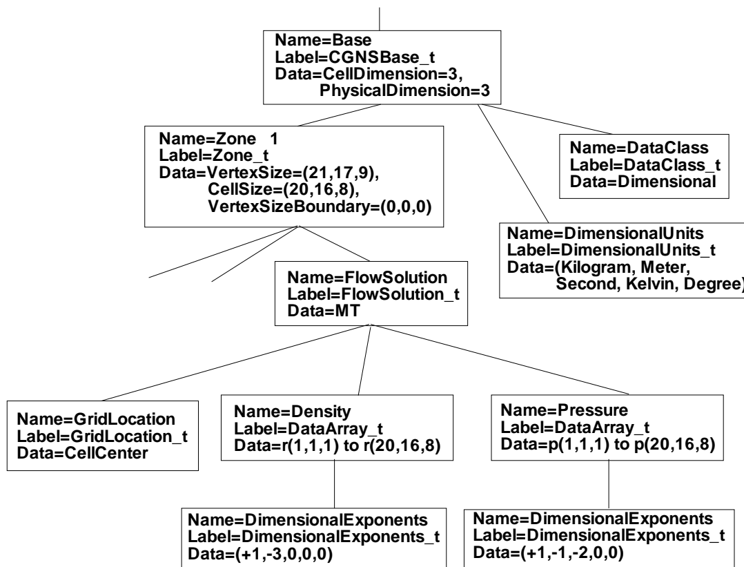
Figure 17: Layout of part of a CGNS file for flow solution at cell centers with dimensional data.
